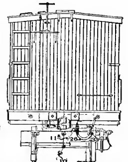
Fig 1695. End Elevation.
